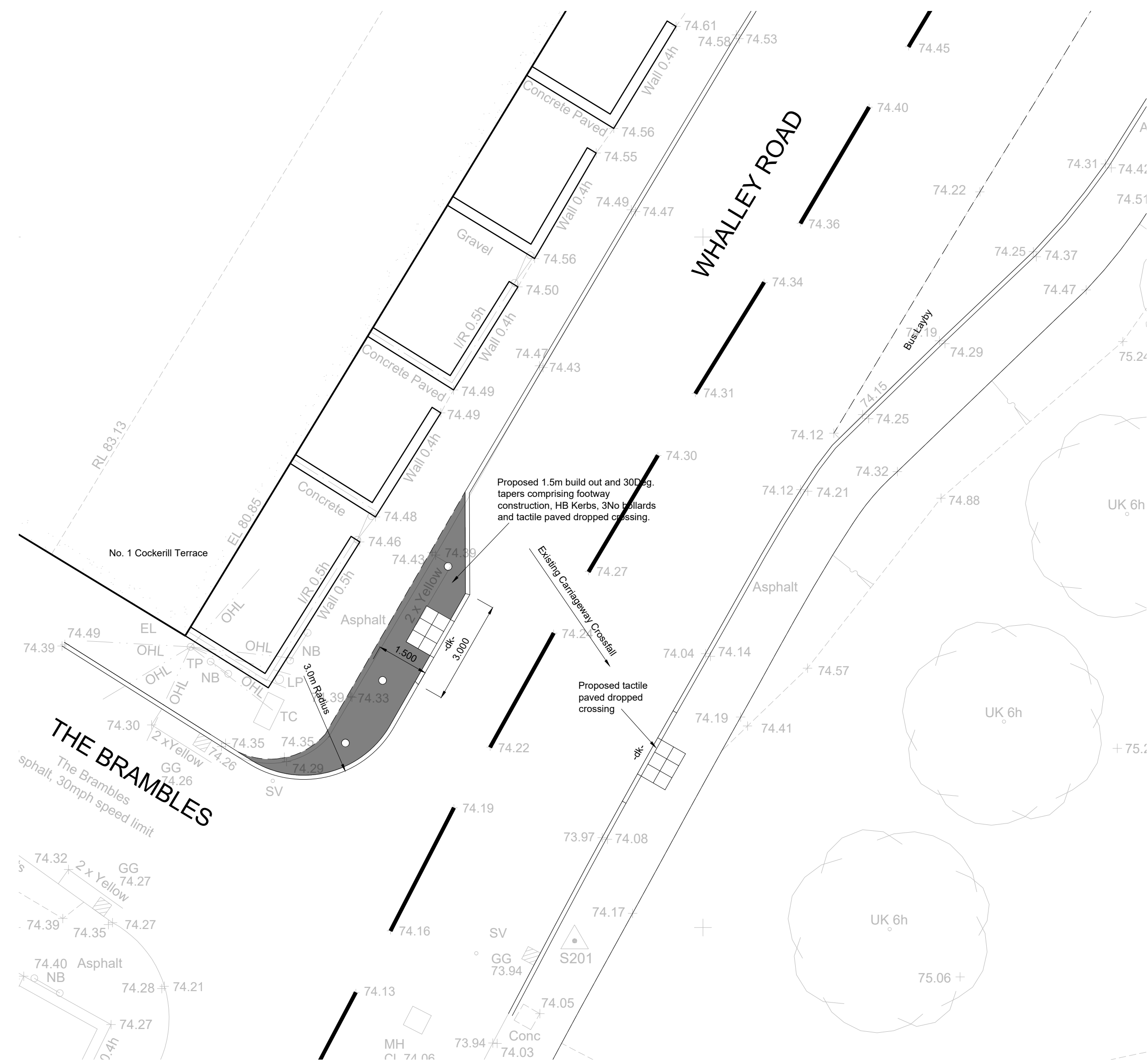
Proposed Whalley Road Traffic Calming GA Plan - 1:100
