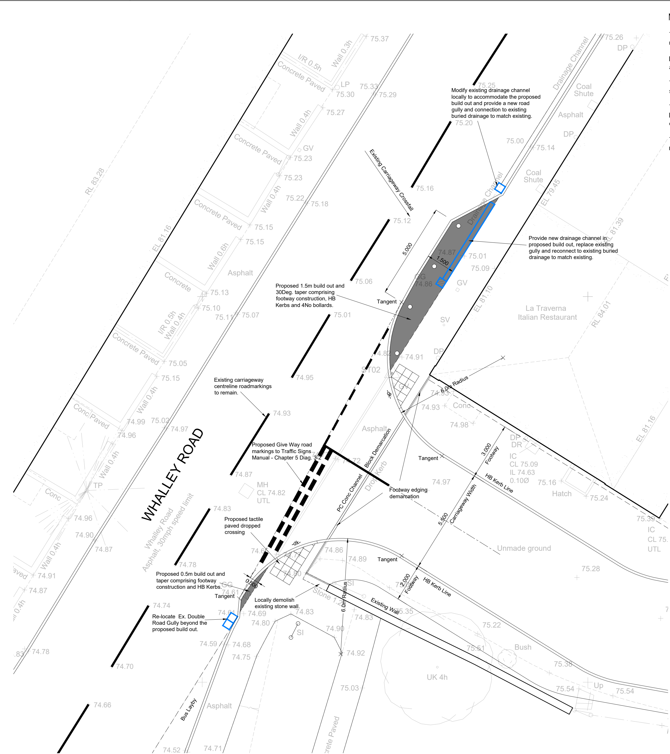
Proposed Whalley Road Traffic Calming And Vehicle Access GA Plan - 1:100
