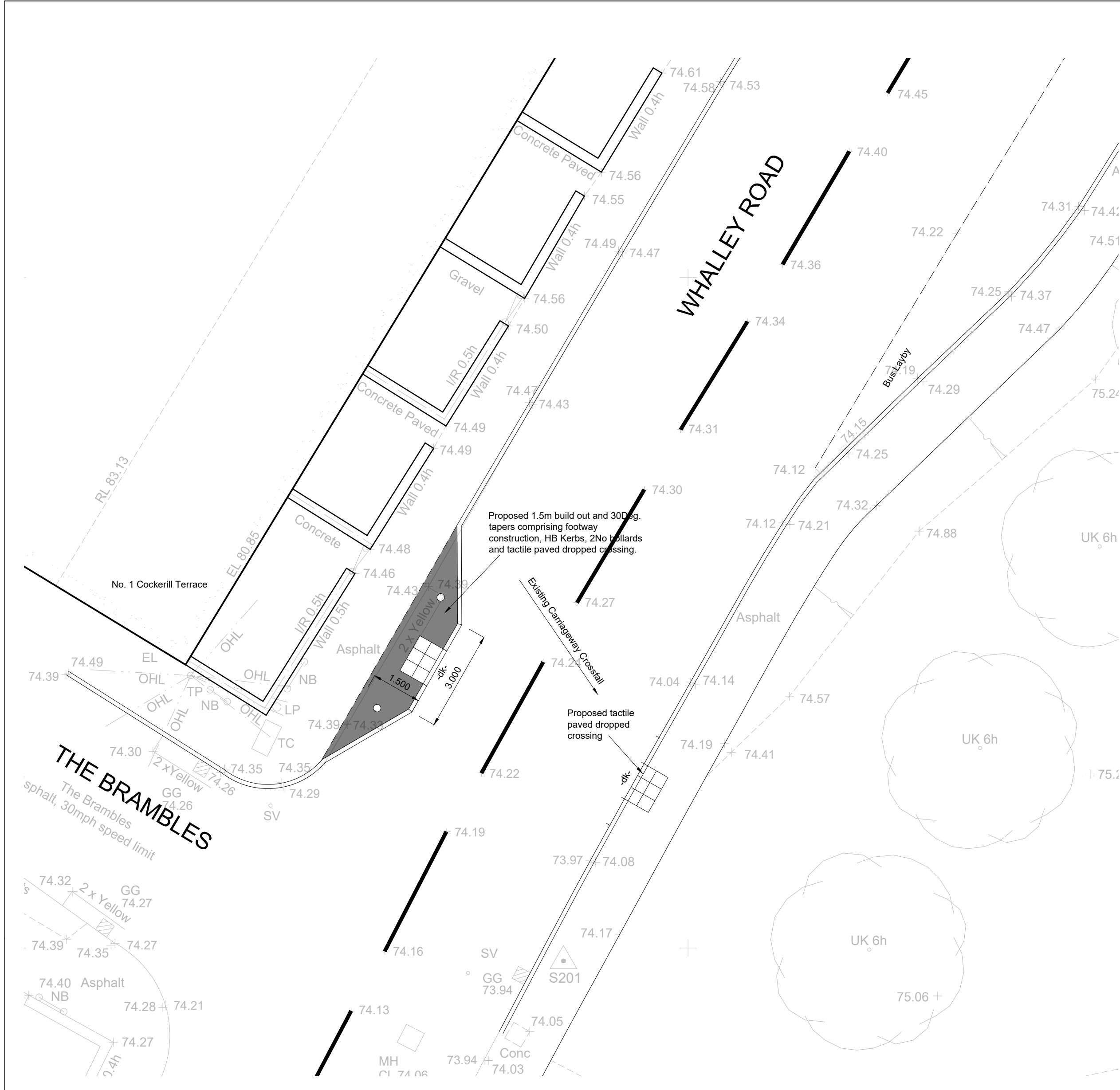
Proposed Whalley Road Traffic Calming GA Plan - 1:100
