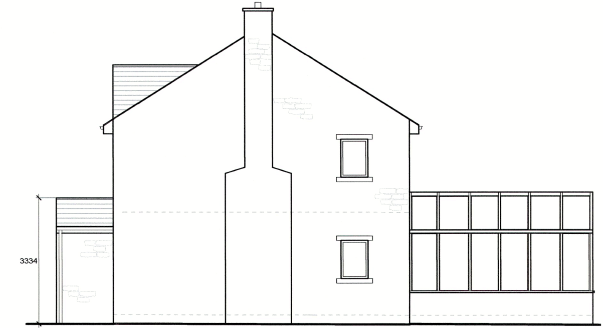
South Elevation 1:100
