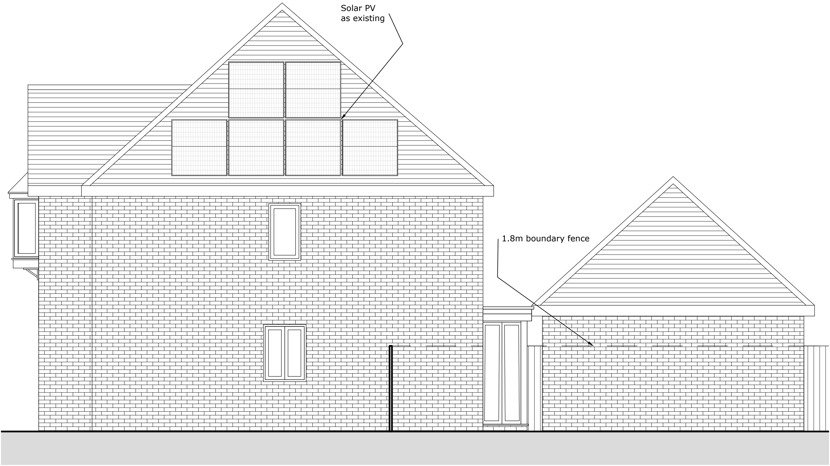
East Elevation as EXISTING 1:50
