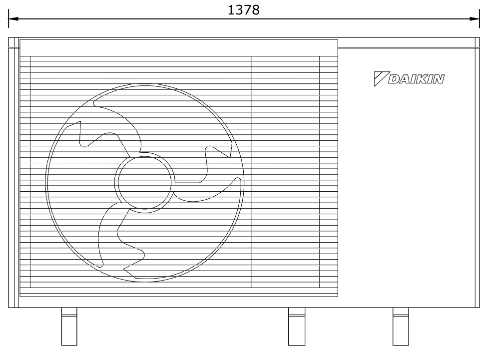
Front view 1:10
