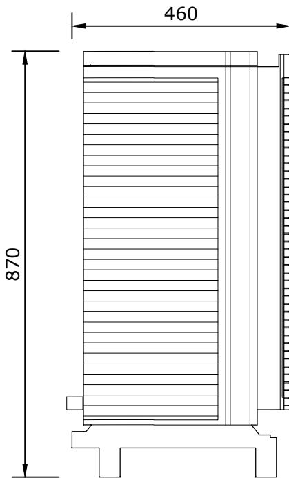
Side view 1:10
