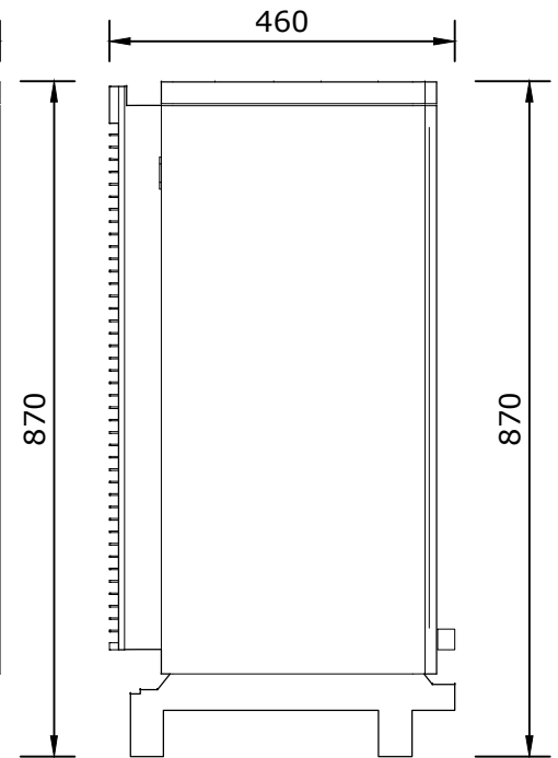
Side view 1:10
