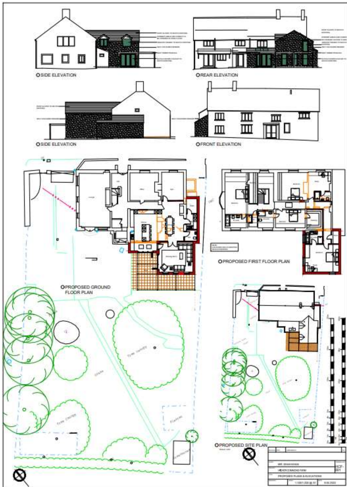
Figure 2: Development Proposals Plan
