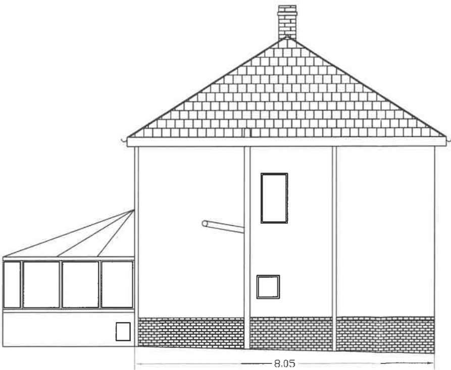
GABLE ELEVATION
