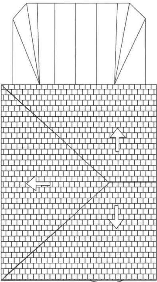
ROOF PLAN
