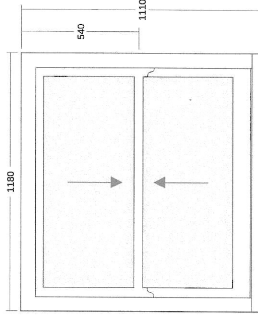
3. Slim Sash Window (Back Bedroom )
