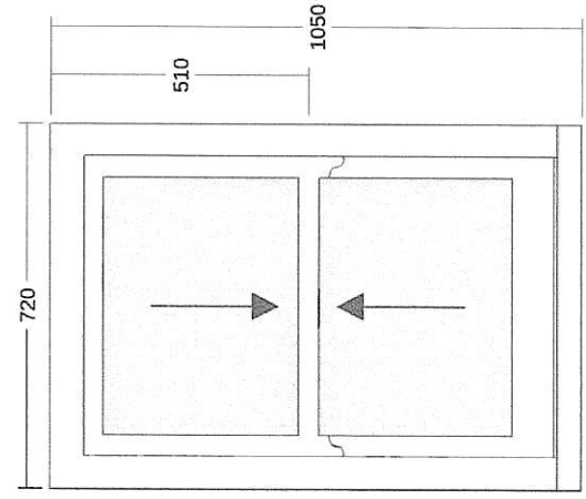
4. Slim Sash Window (Shower Room )
