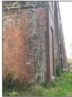
DEFECT DD.03 AREA OF SPALLLED BRICKWORK
