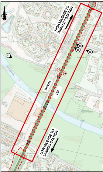
SITE PLAN SCALE 1:50,000
