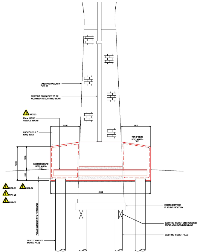
TYPICAL SECTION THROUGH BORED PILE RING BEAM SCALE: 1:25
