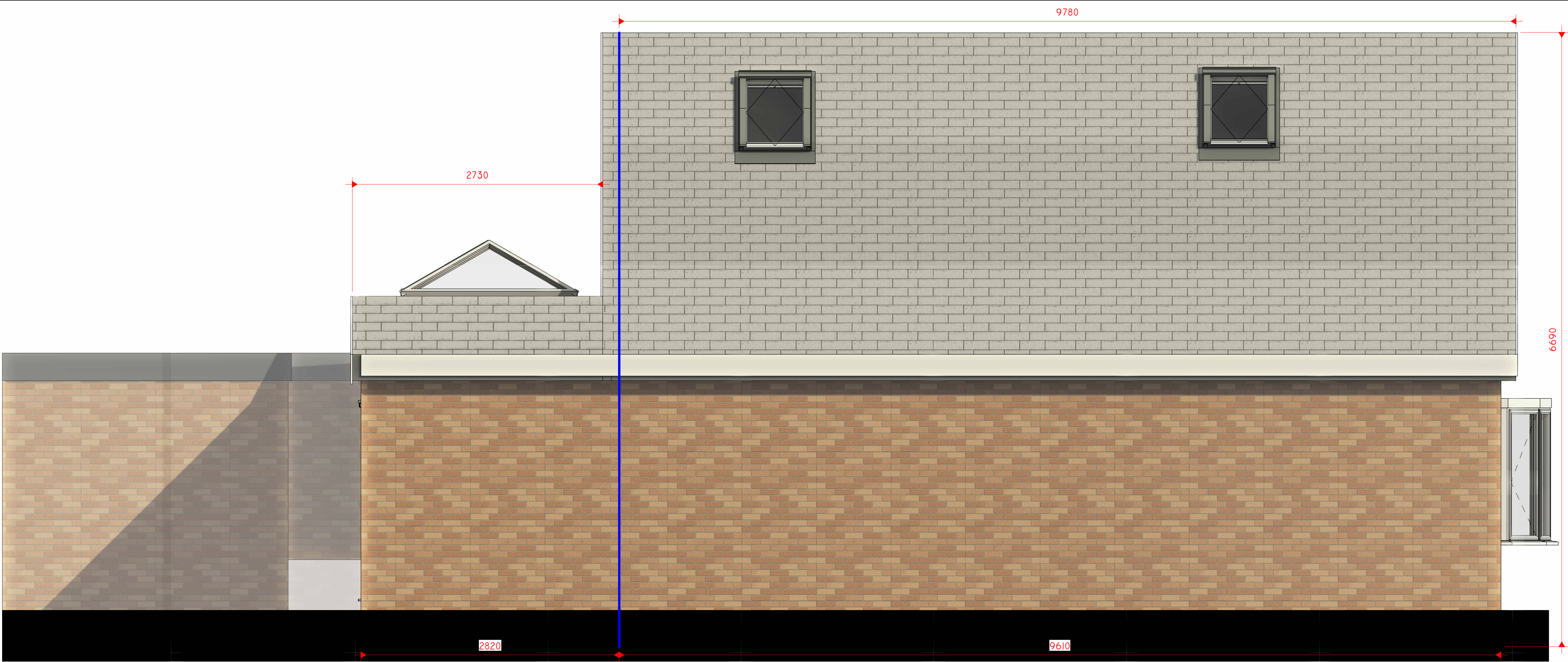
1 PROPOSED SOUTH 1 : 25
