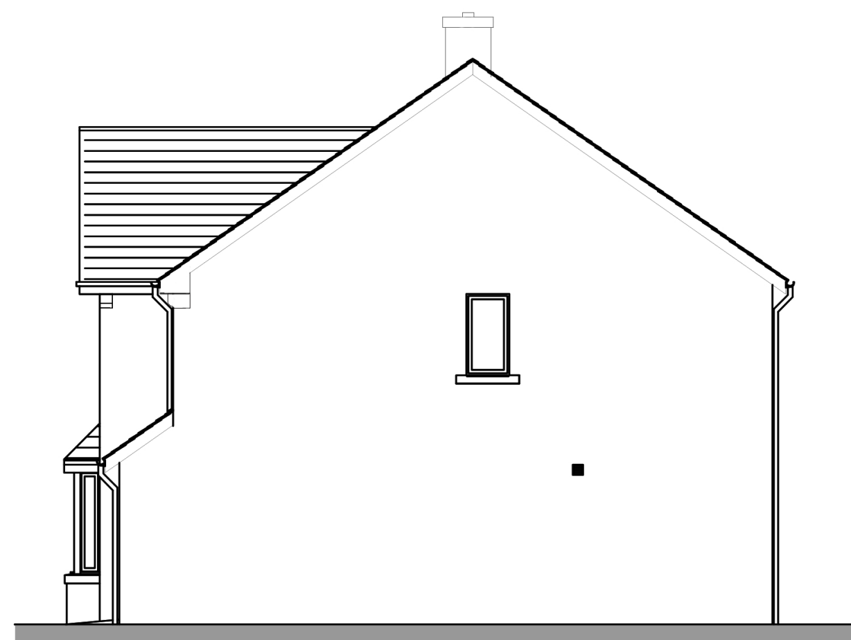
SIDE ELEVATION
