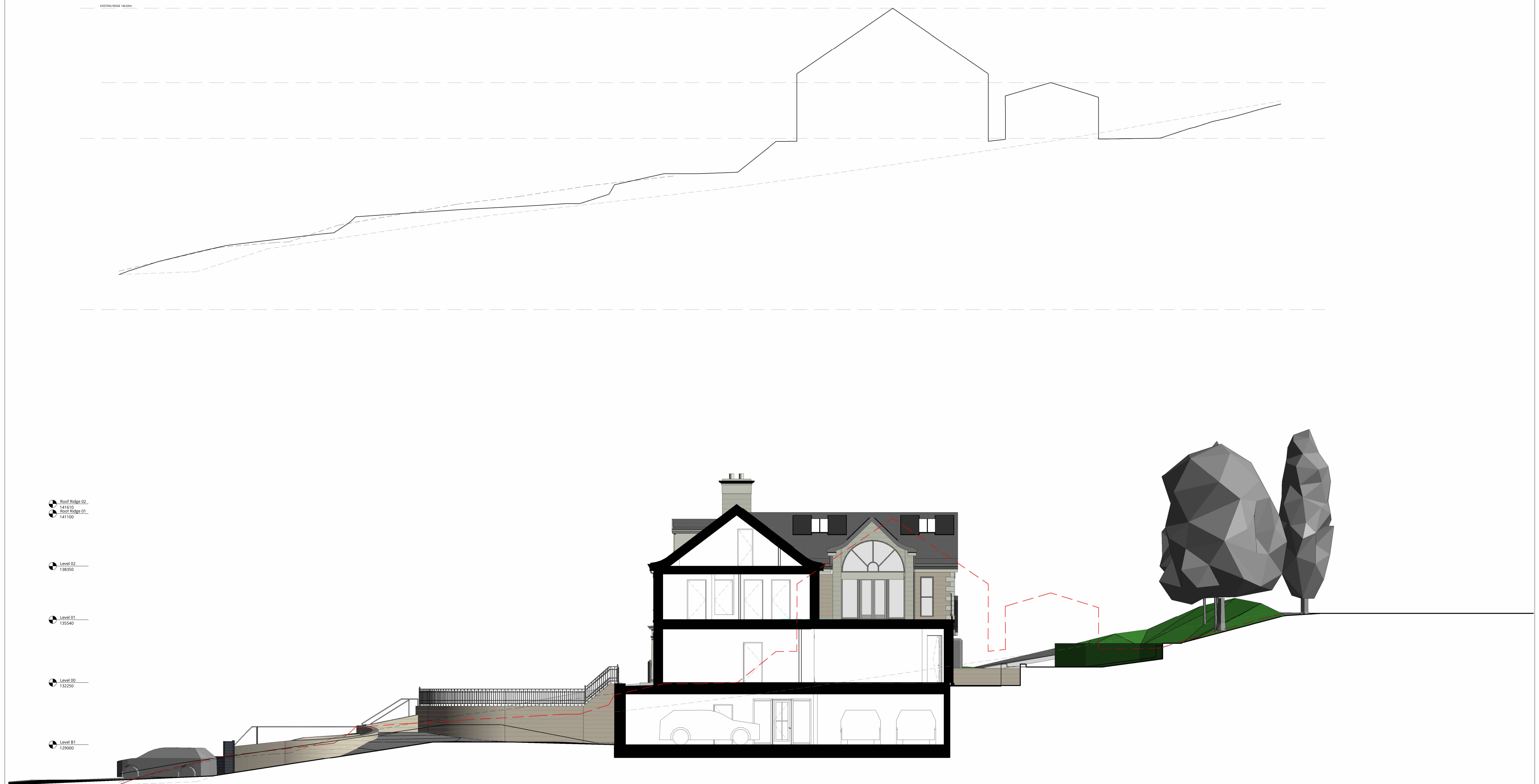
1 Existing & Proposed Section 1 : 100
