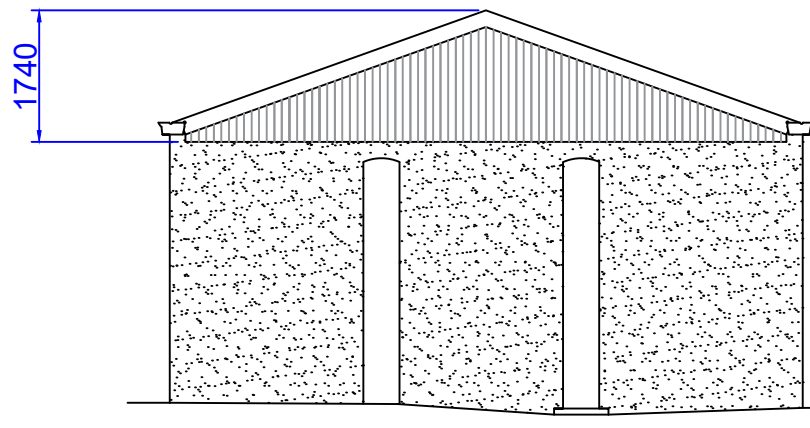
Side Elevation (2)
