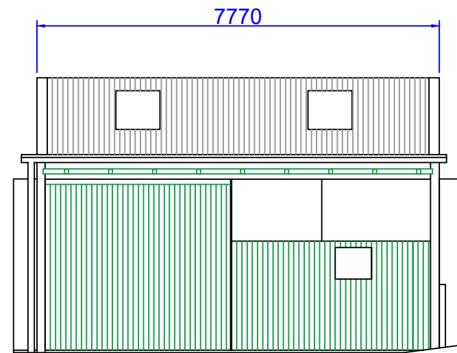
Front Elevation
