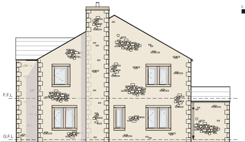
South Elevation
