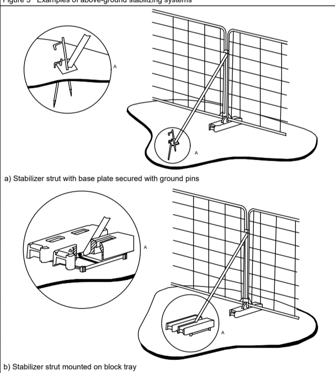
BS5837:2012 Figure 3 Examples of above-ground stabilizing systems
