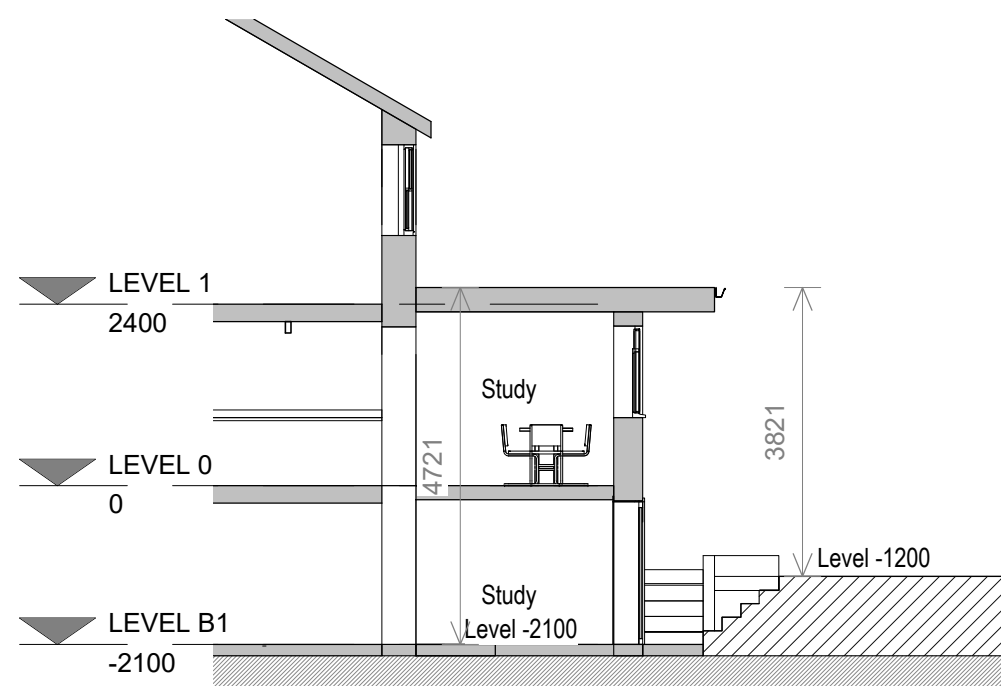
1 Proposed Section 1 : 100
