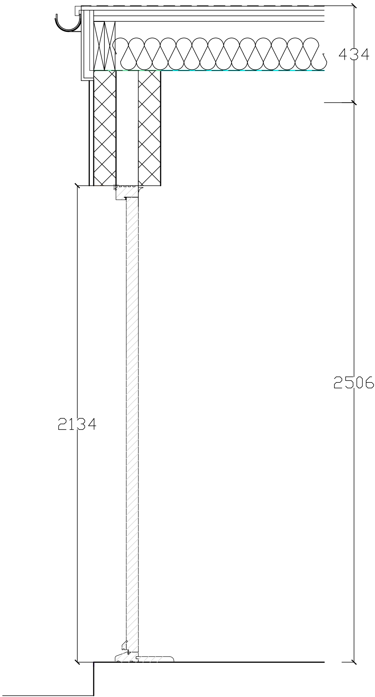
EXISTING SECTION A- (1:10)
