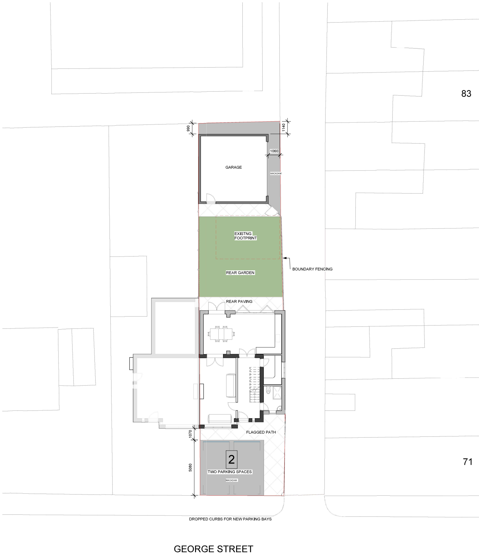
1 PROPOSED SITE PLAN 1 : 100
