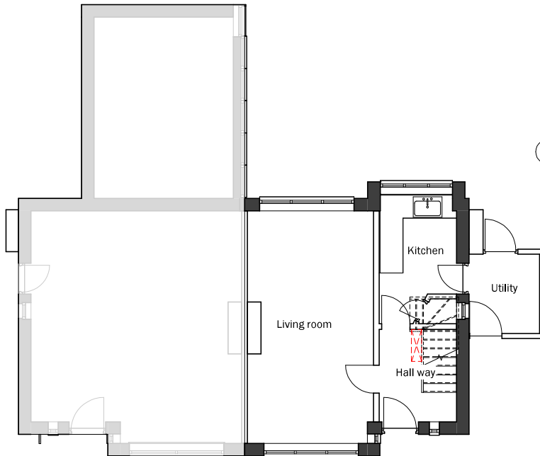
1 0 GROUND FLOOR 1 : 50
