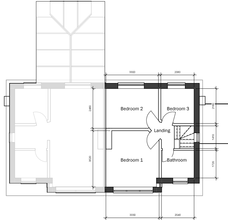
2 1 FIRST FLOOR 1 : 50
