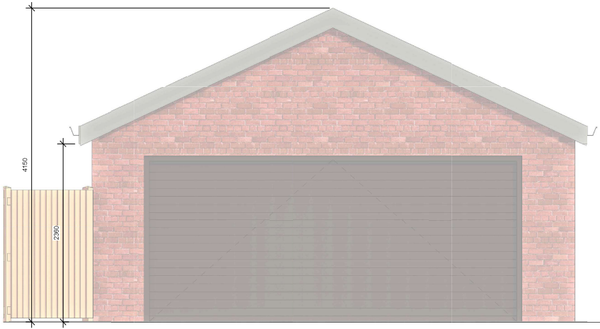
2 PROPOSED EAST 1 1 : 25
