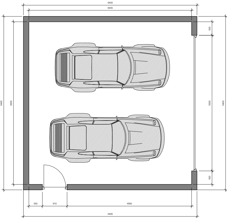
1 PROPOSED GARAGE FLOOR 1 : 25
