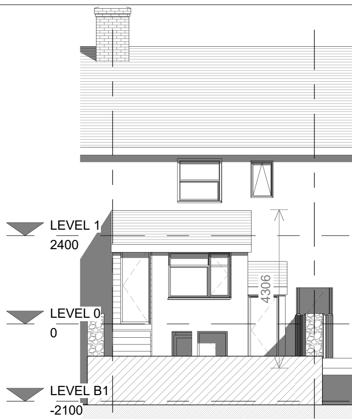
3 Rear - Existing 1 : 100
