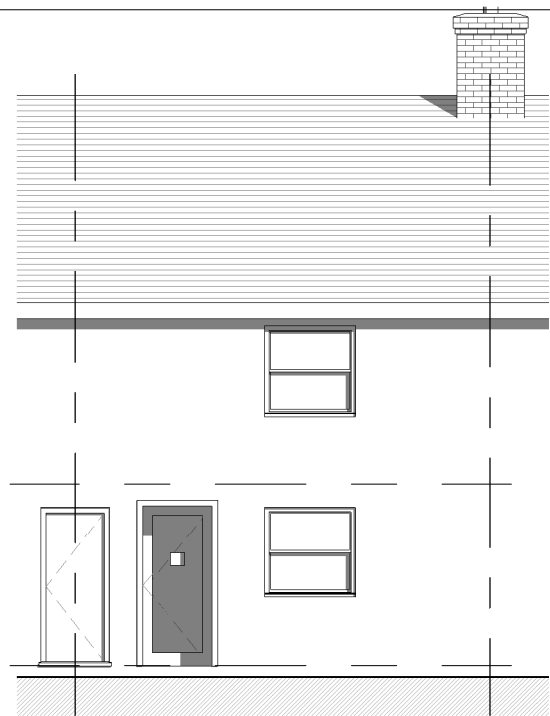
1 Front - Existing 1 : 100
