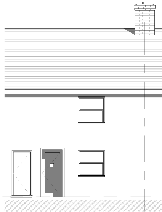
1 Front - Proposed 1 : 100
