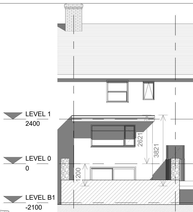
3 Rear - Proposed 1 : 100
