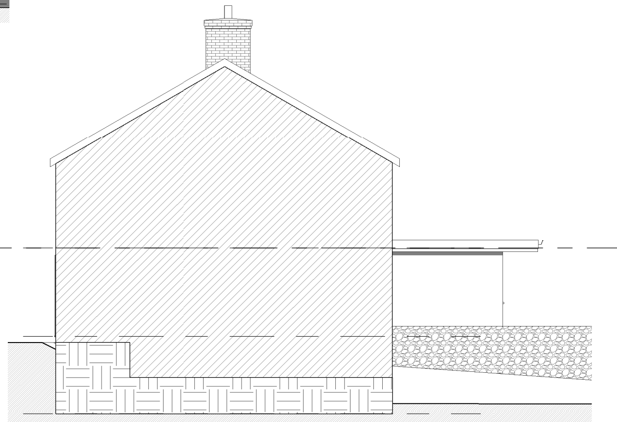
4 Right Side - Proposed 1 : 100
