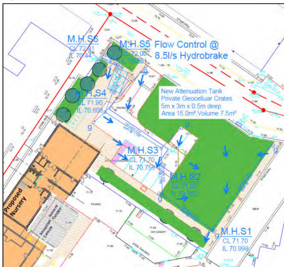
Figure 2-6: Phase 2 Drainage Plan
