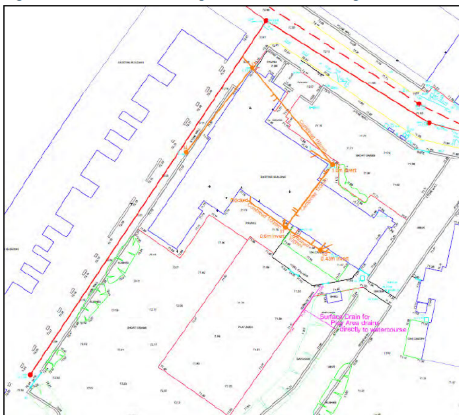
Figure 2-3: Sketch of Existing Infant School Drainage
