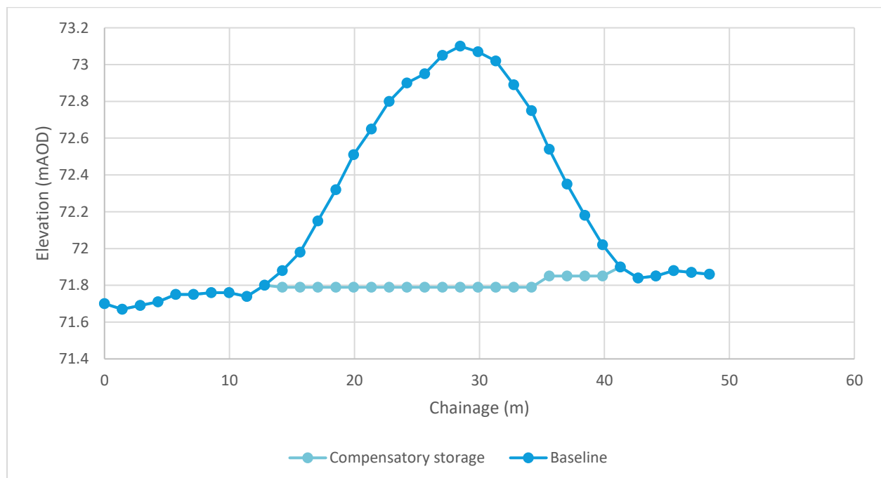
Figure 7-4: Cross Section Profile - A
