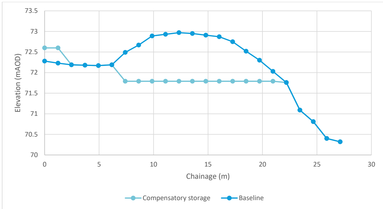
Figure 7-5: Cross Section Profile - B
