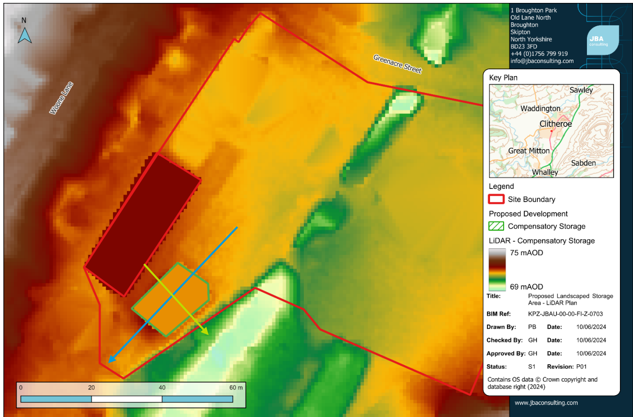
Figure 7-3: Proposed landscape storage area - LiDAR Plan. Cross section A (Blue), B (Green)
