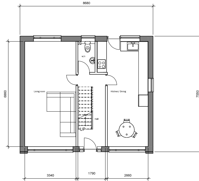
1 0 GROUND FLOOR 1 : 50
