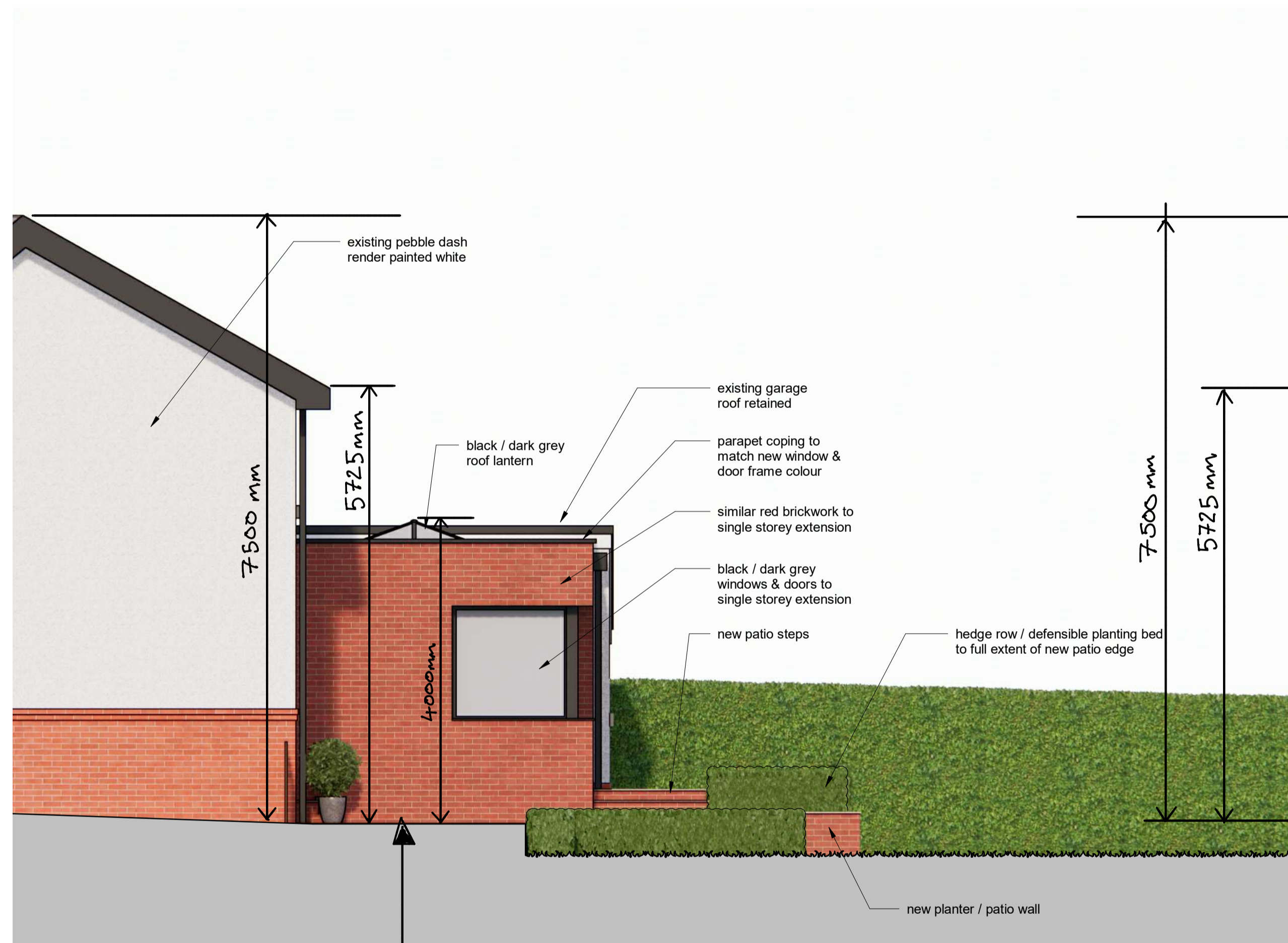
Proposed Side Elevation 1:50
