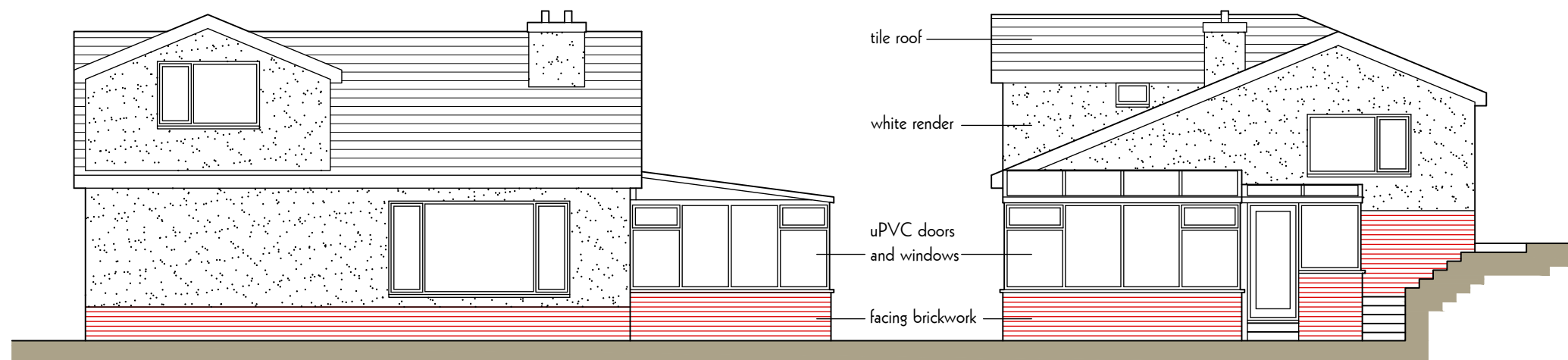
West Elevation
