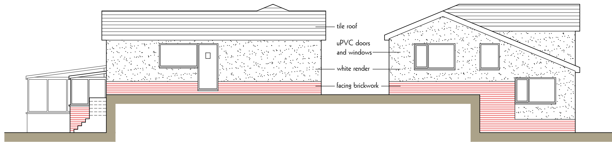
East Elevation
