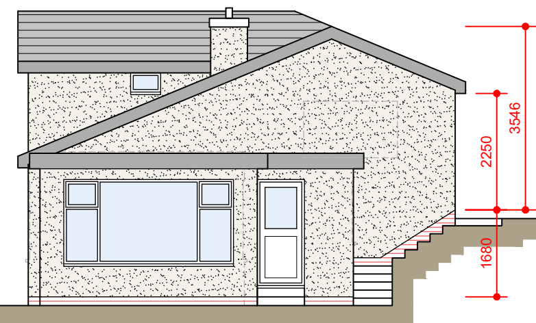
South Elevation
