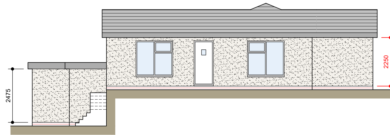
East Elevation
