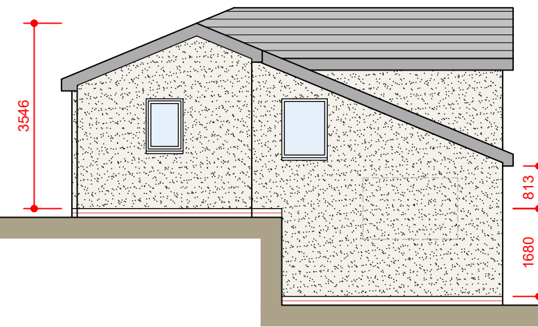
North Elevation
