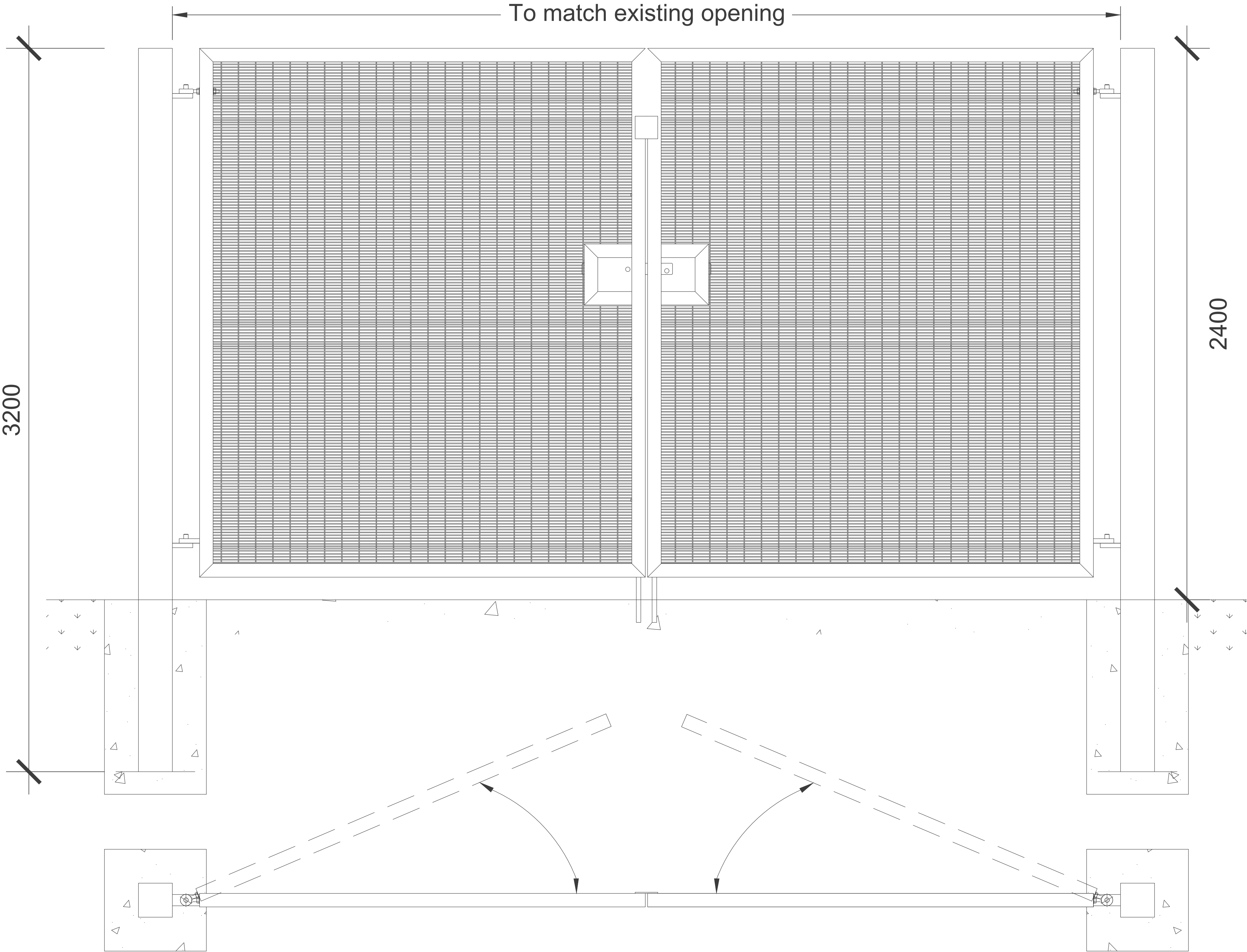
Fencing Elevations Scale 1:10 @ A1
