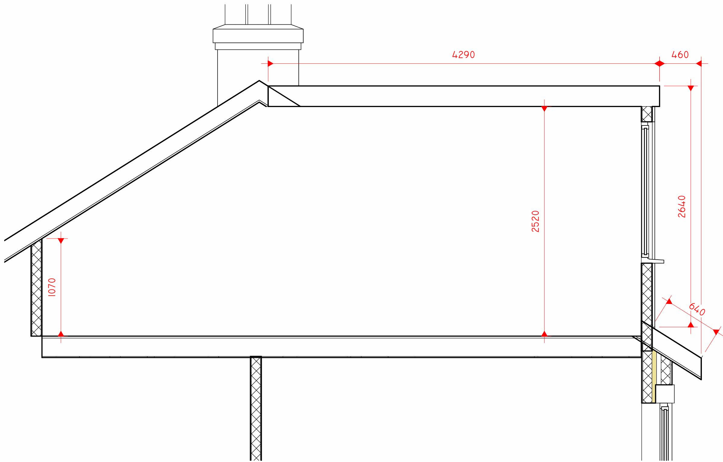
1 DORMER CUT SECTION 1 : 25
