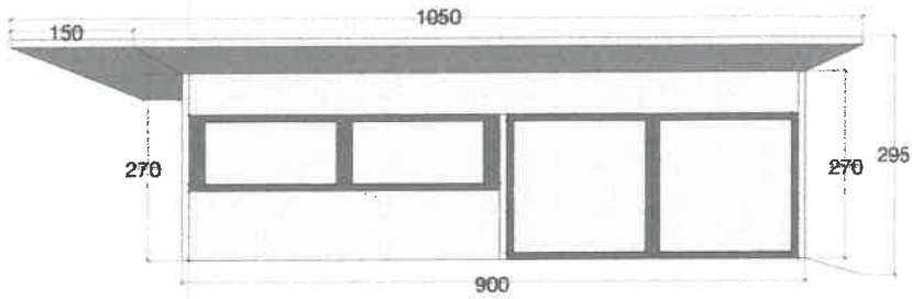
Stable - Proposed Easterly Facing Elevation - 1:100
