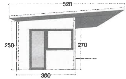
Stable - Proposed Sotherly Facing Elevation - 1:100
