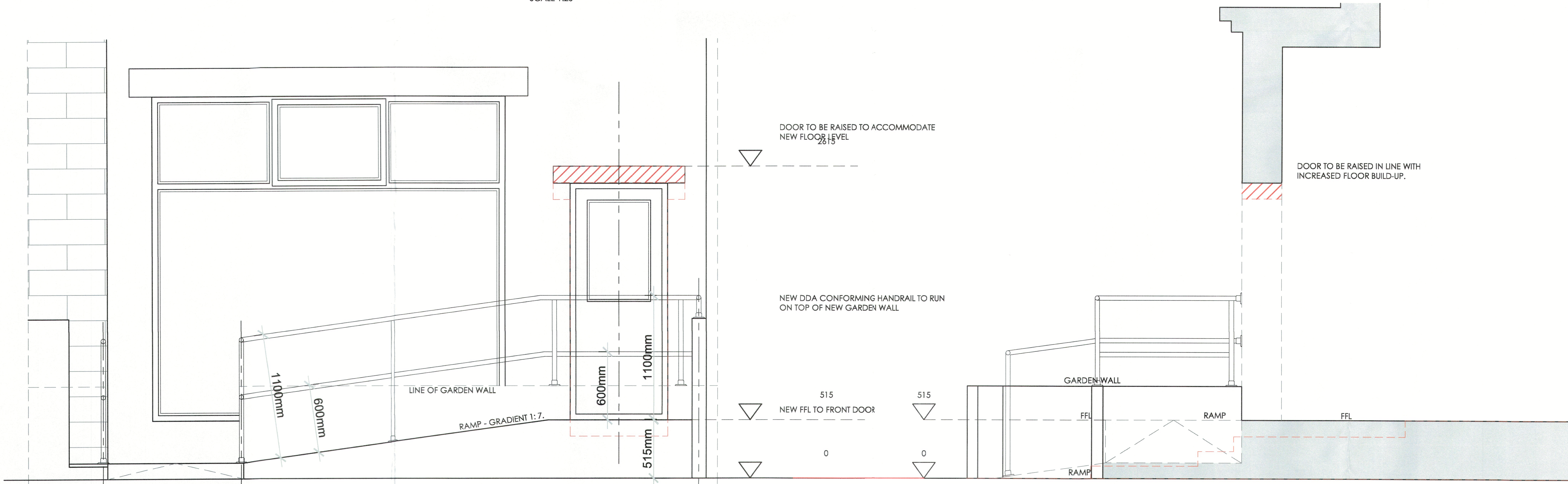
RAMP ELEVATION - SCALE 1:20
