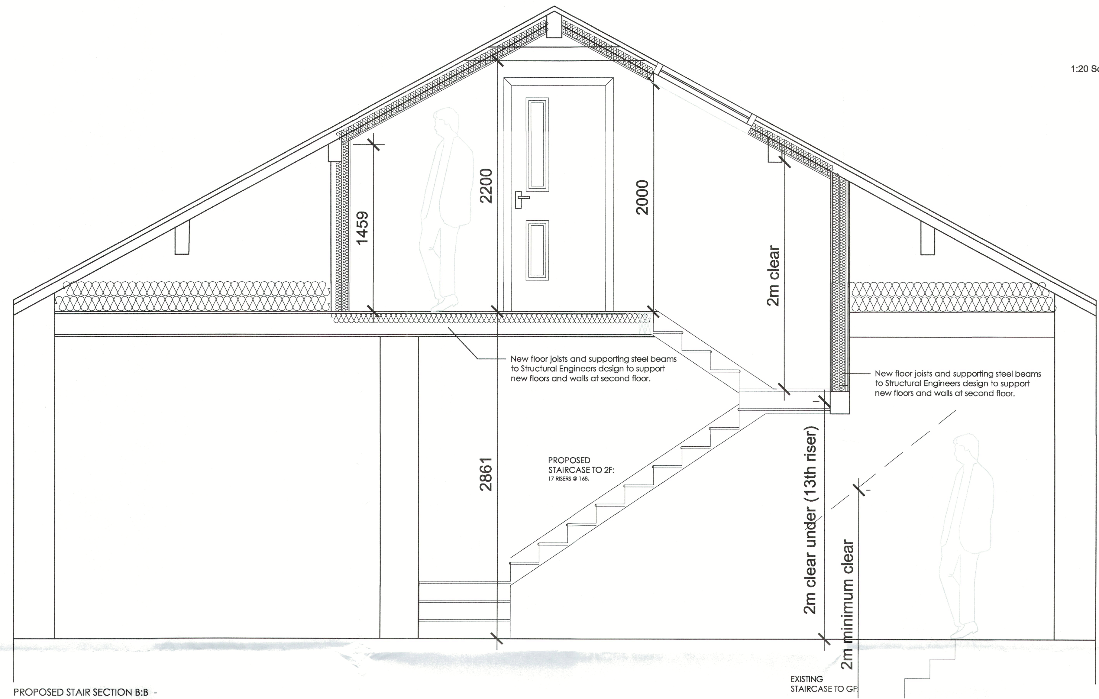
PROPOSED STAIR SECTION B:B - SCALE 1:20
