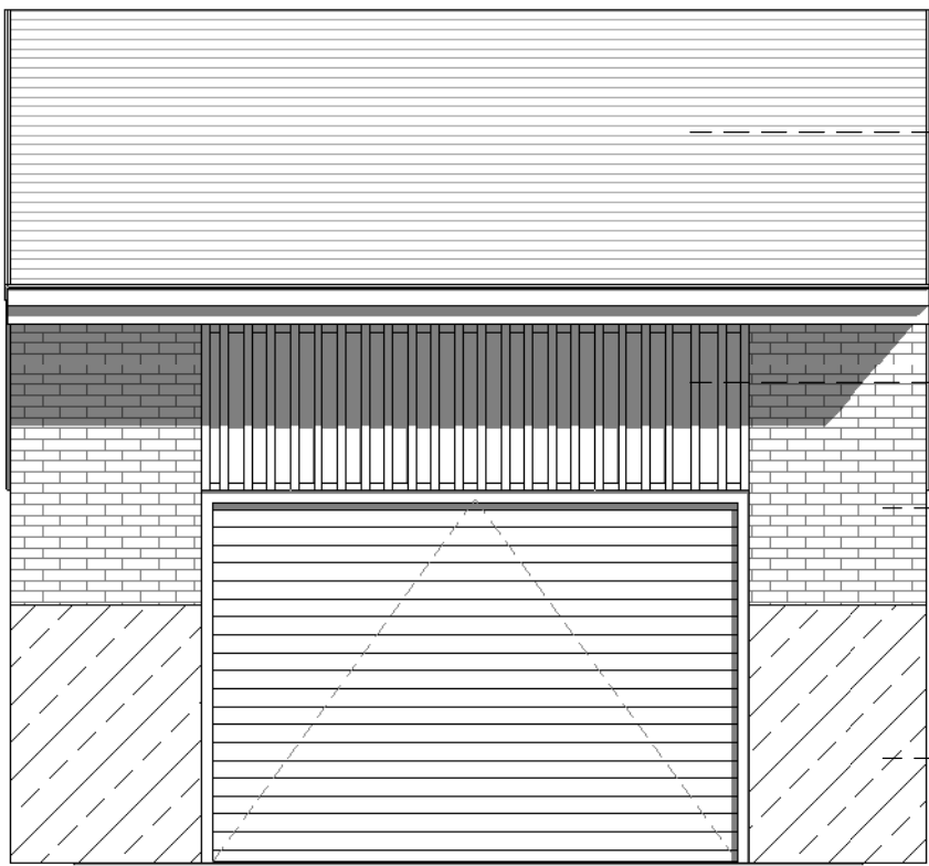
2 Front Elevation 1 : 50
