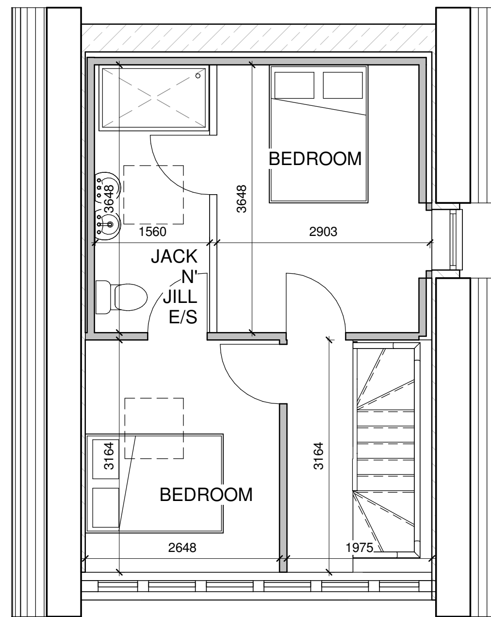
7 Mezzainine Level 1 : 50
