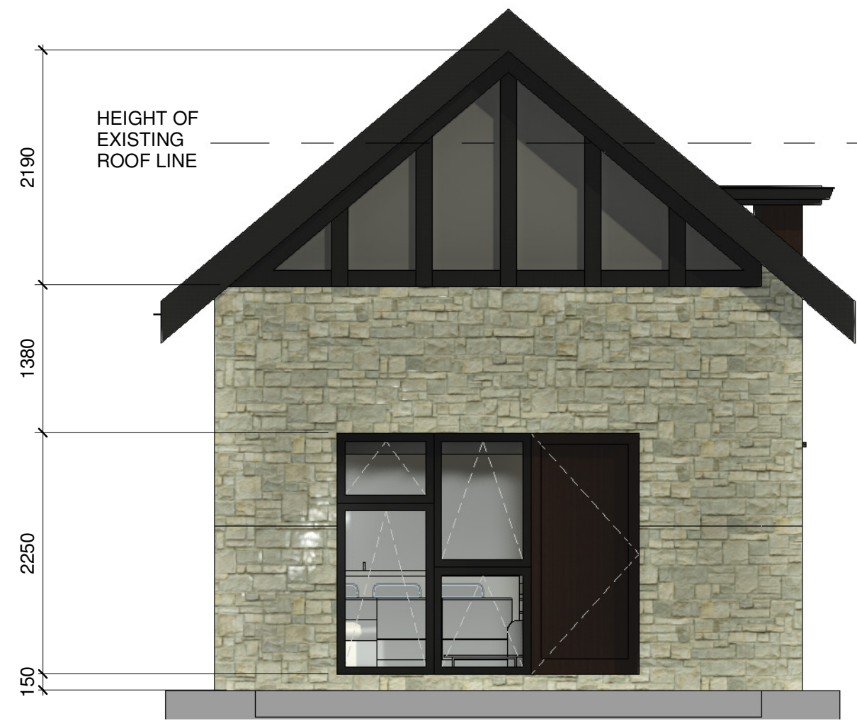
2 Front Elevation 1 : 50
