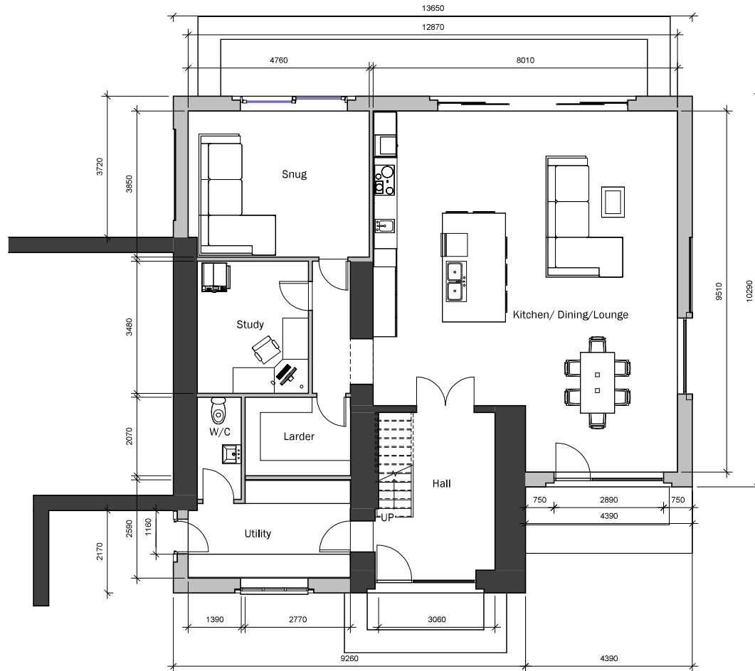
1 0 PROPOSED GROUND FLOOR 1 : 50
