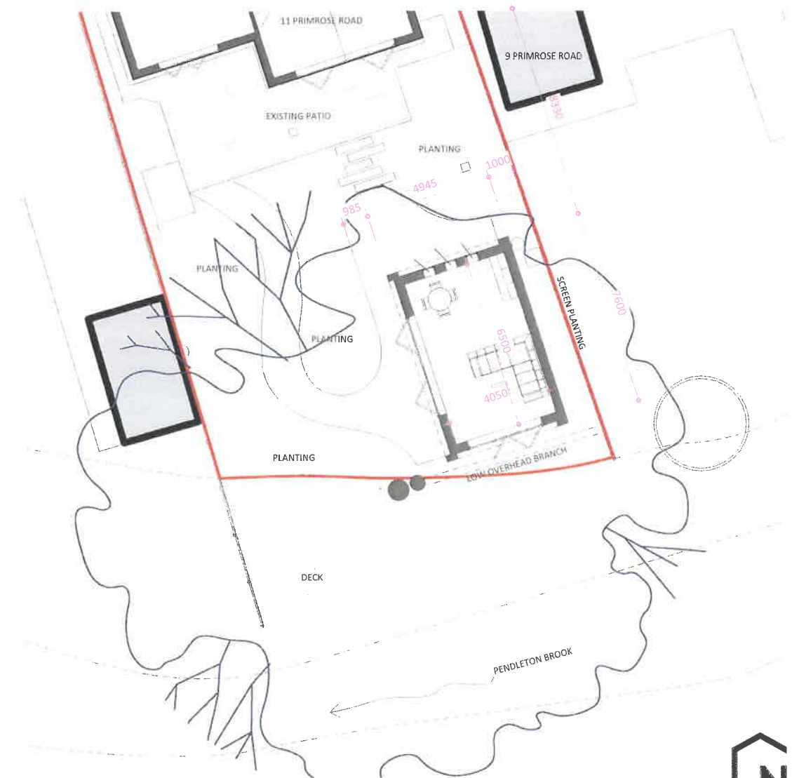
1 PROPOSED GROUND FLOOR 1:100
