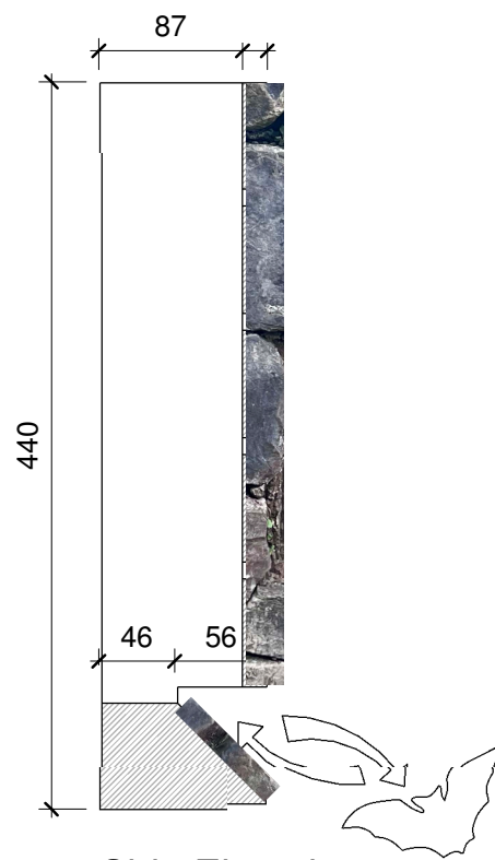
Side Elevation
