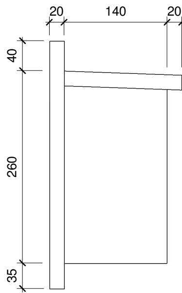
Side Elevation
