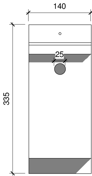
Front Elevation
