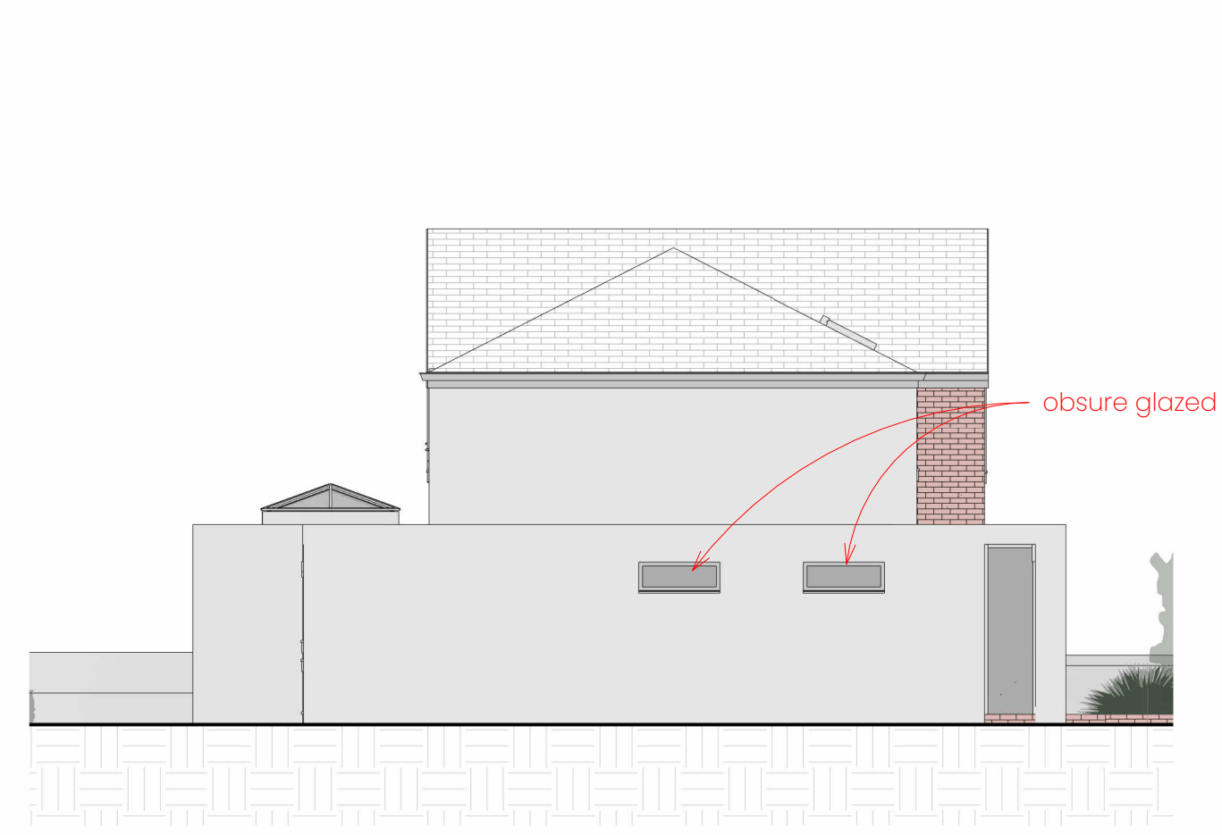
6 Proposed North West 1:100
