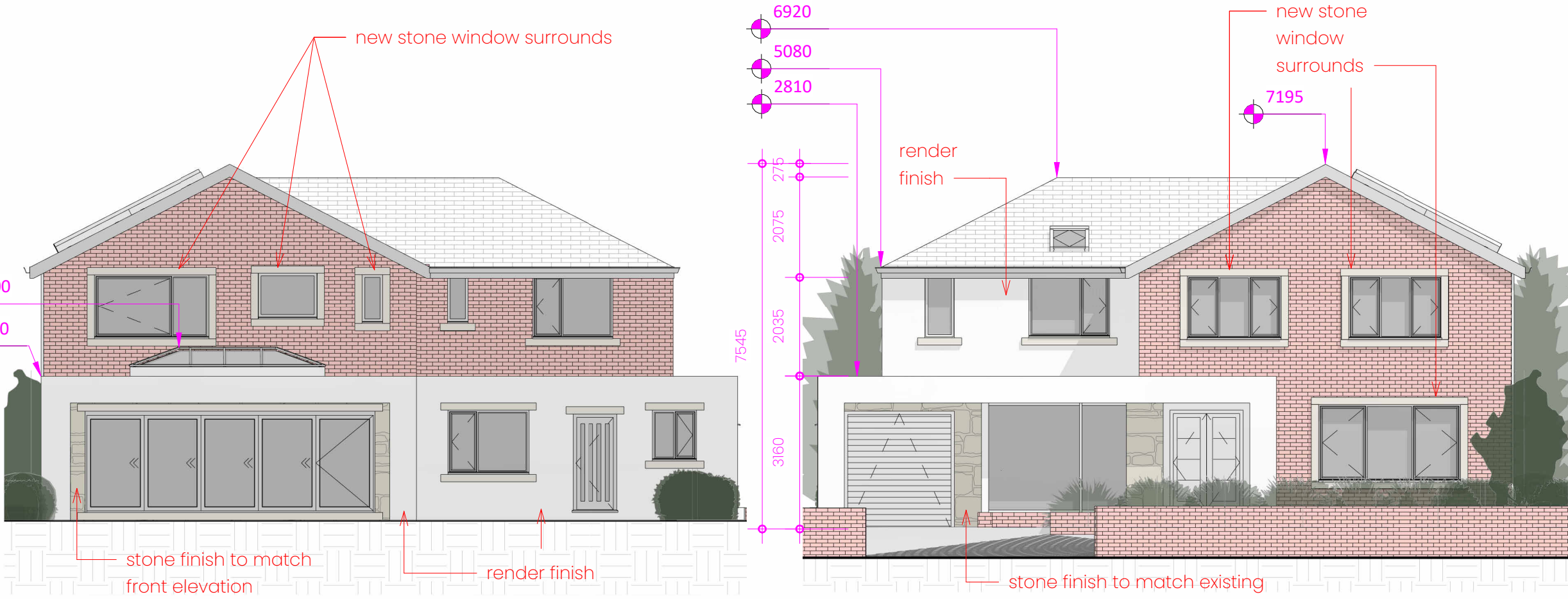
5 Proposed South West 1:100
