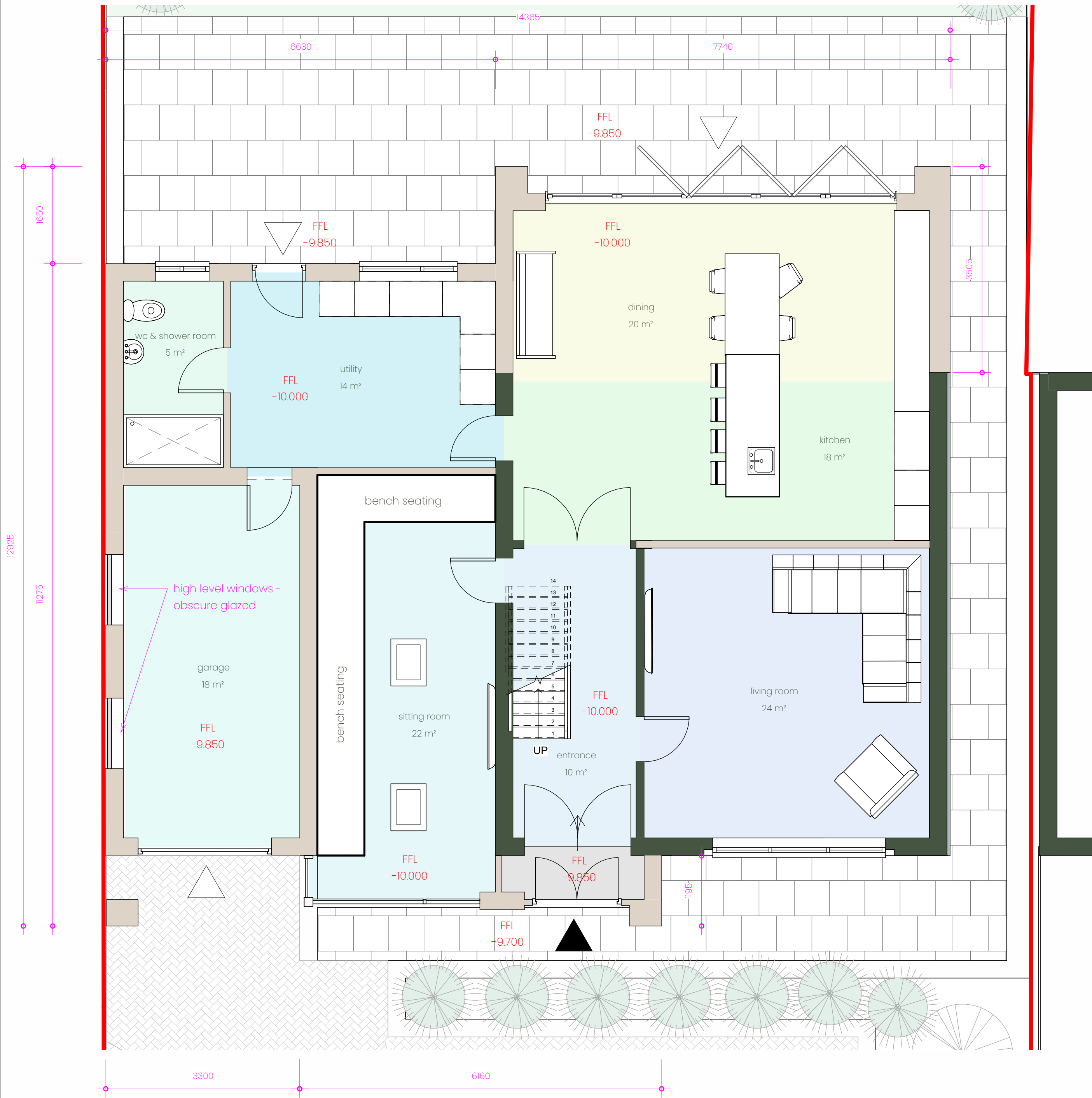
1 Proposed Ground floor 1:50
