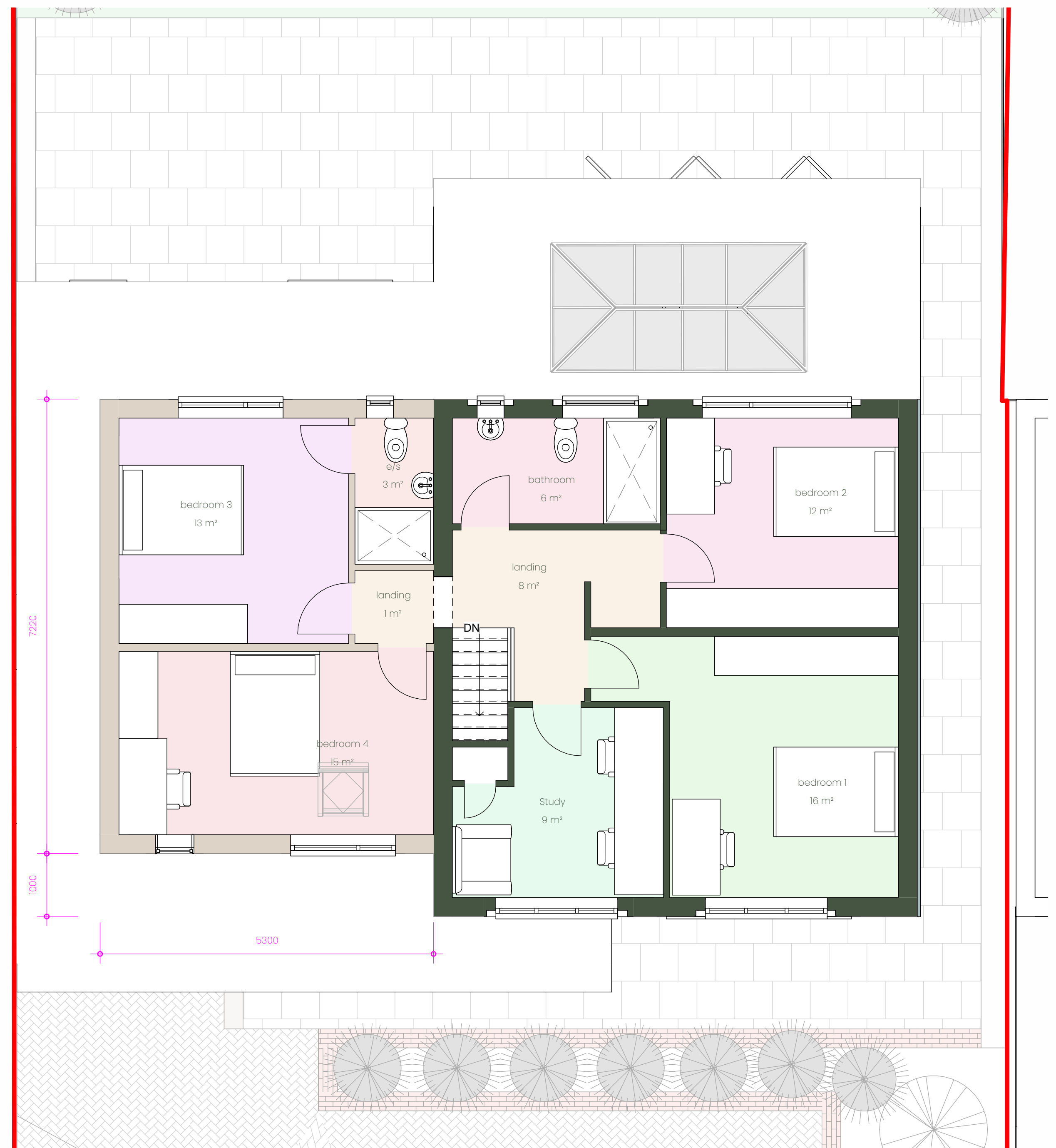
2 Proposed First floor 1:50
