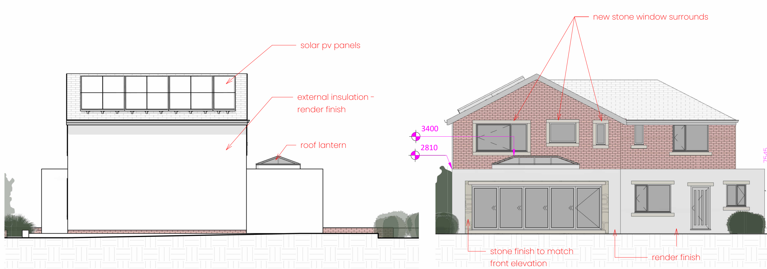
3 Proposed South East 1:100
