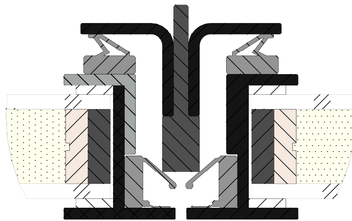
DETAIL B SCALE 1 : 1
