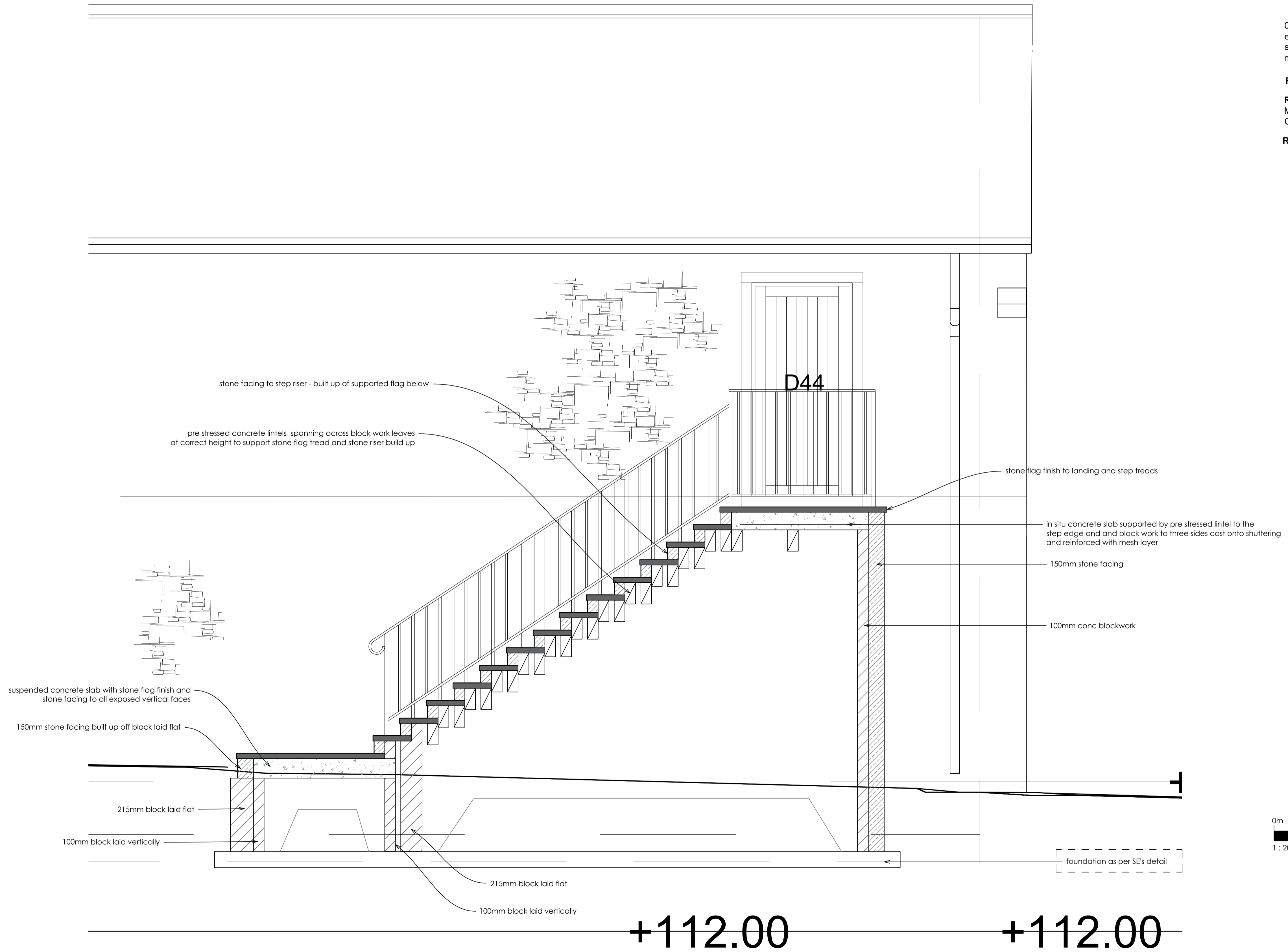
TYPICAL SECTION TO EXTERNAL STAIRS
