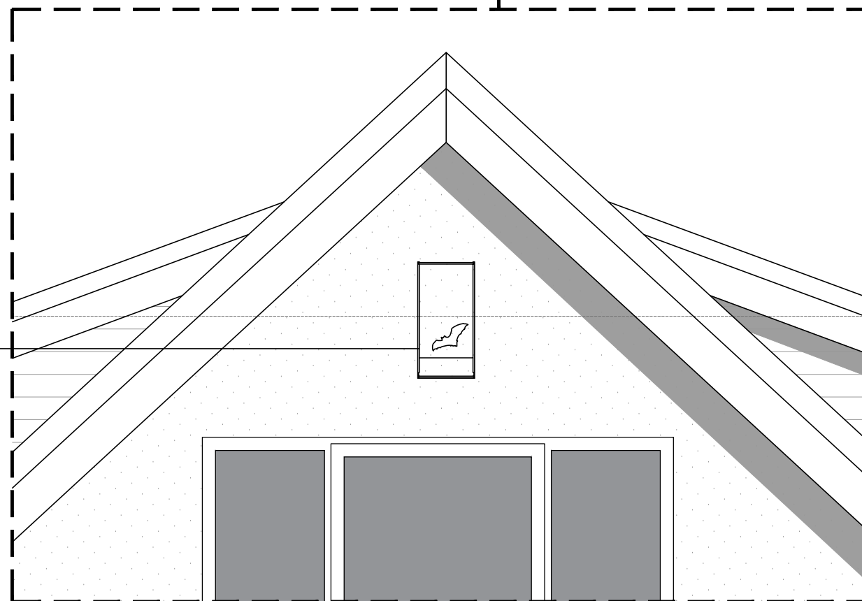
Front Elevation Detail 1:20
