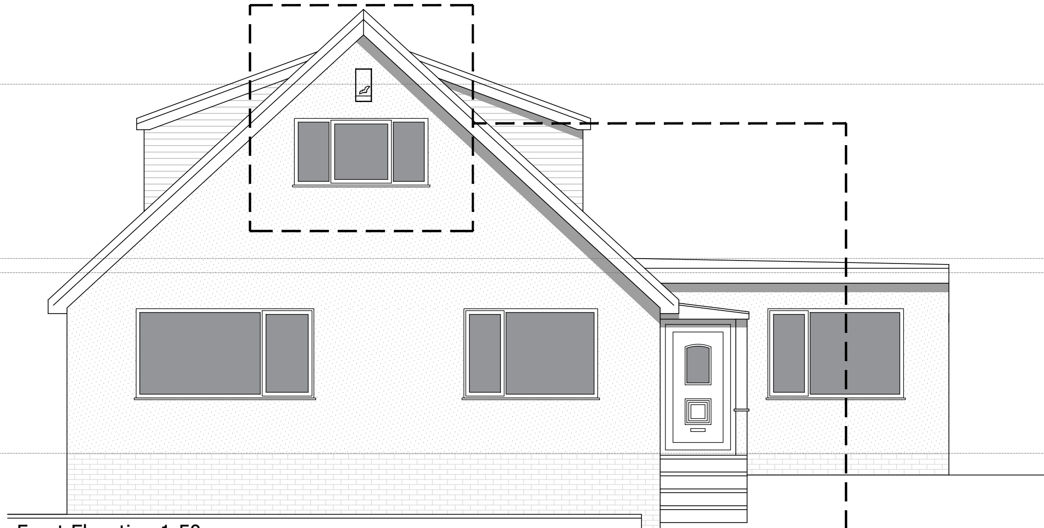
Front Elevation 1:50
