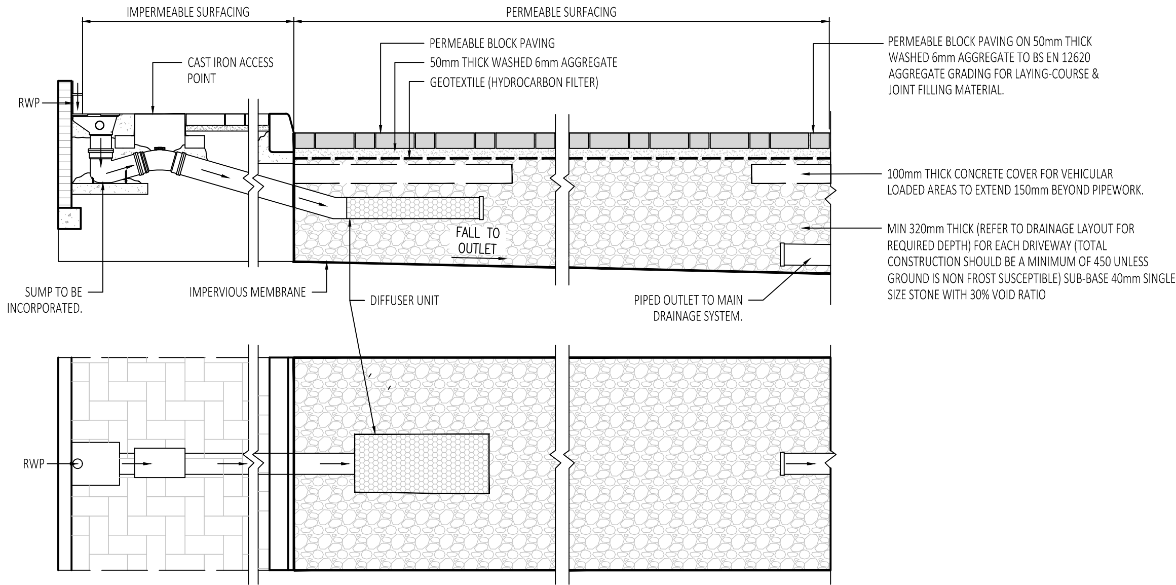
TYPICAL SECTION THROUGH PIPED OUTFALL INTO PERMEABLE PAVING SUB-BASE USING DIFFUSER UNITS 1:20mm
