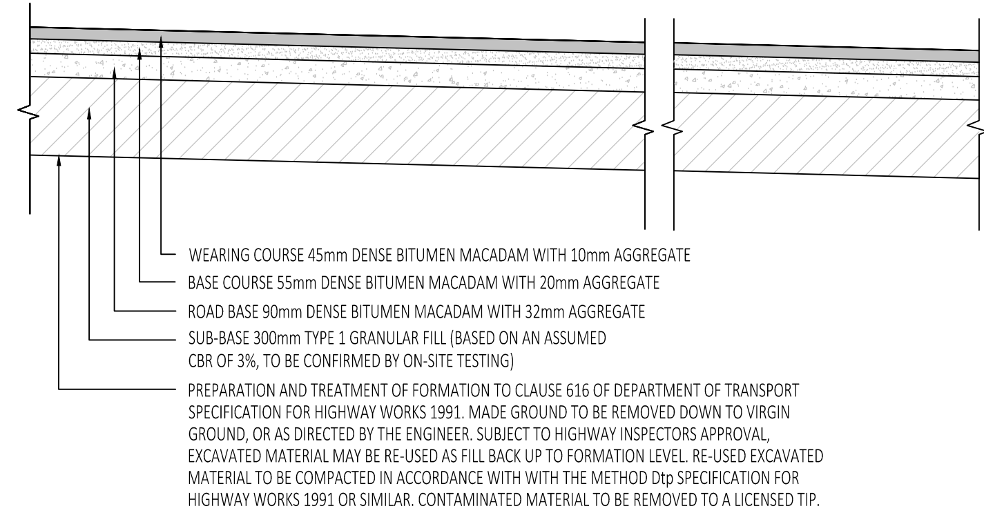
DRIVEWAY OPTION 1 (1:20)
