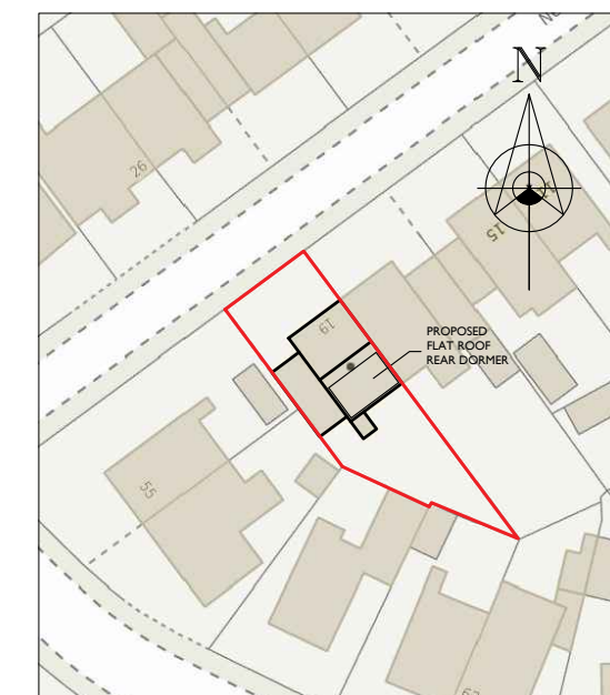
PROPOSED SITE PLAN 1:500
