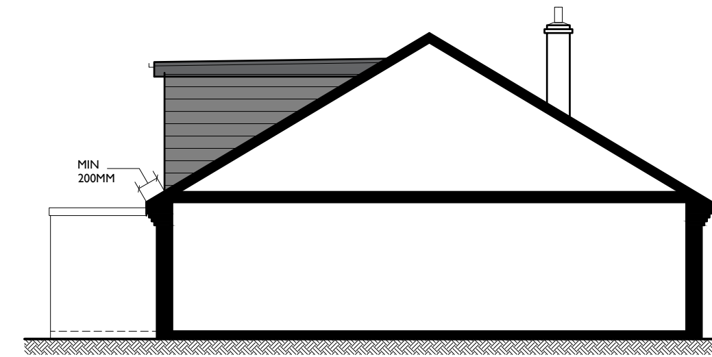
PROPOSED SIDE SECTIONAL ELEVATION 1:100
