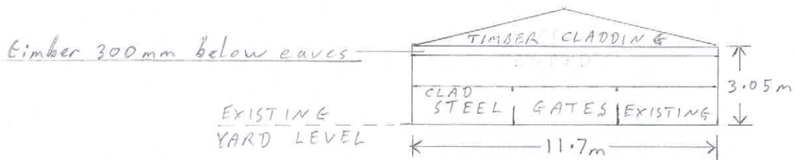
SOUTH WEST ELEVATION
