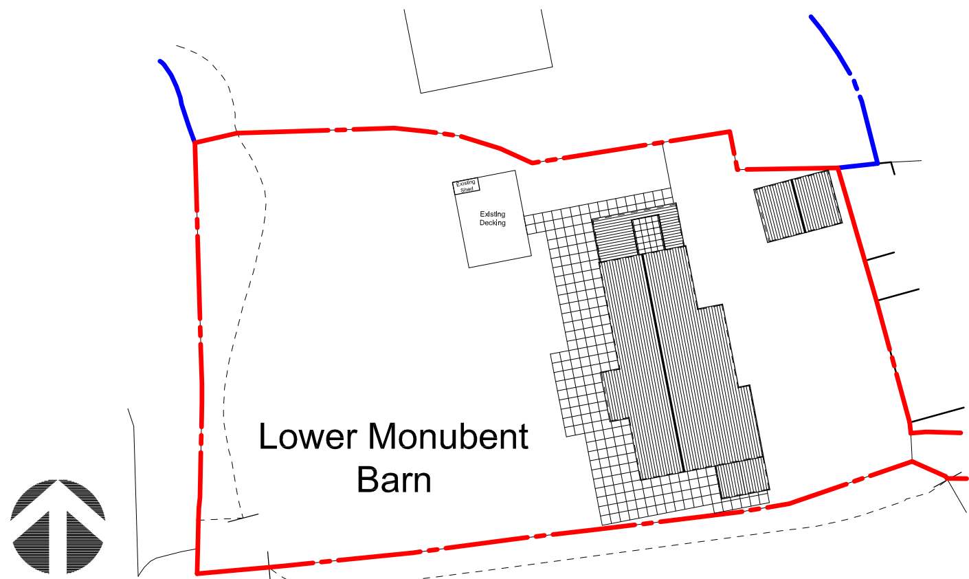
EXISTING BLOCK PLAN Scale: 1:500 at A1
