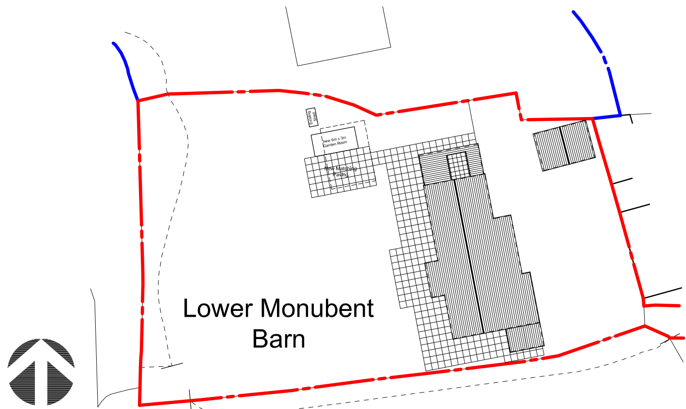
PROPOSED BLOCK PLAN Scale: 1:500 at A1
