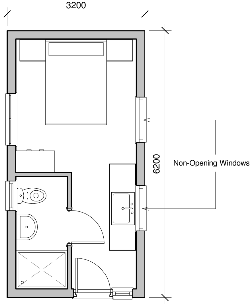
FLOOR PLAN 1:50
