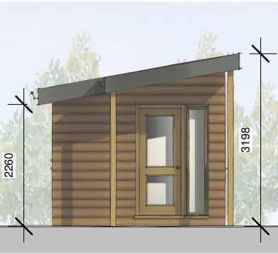
FRONT ELEVATION 1:100
