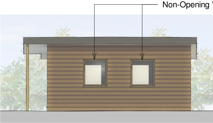
SIDE ELEVATION 1:100
