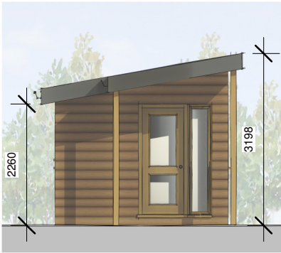
FRONT ELEVATION 1:100
