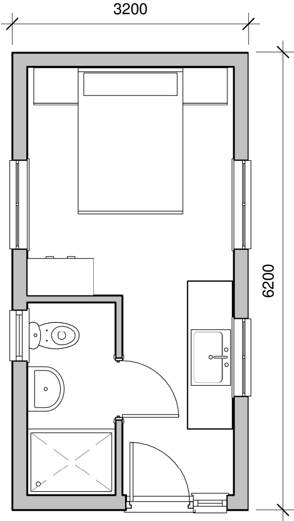
FLOOR PLAN 1:50
